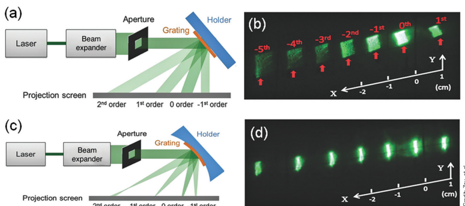
Figure 5. (a) and (c) Schematic diagrams illustrating the experimental setup used to map diffraction patterns from flexible gratings that were attached onto (a) a flat sample holder and (c) a curved sample holder. (b) and (d) Diffraction patterns of a collimated and expanded 532-nm green laser beam by gratings mounted on (b) a flat surface and (d) a curved surface. (Images courtesy of Y. Zou, et al., Adv. Opt. Mater. 2 , 759-764 (2014)).
