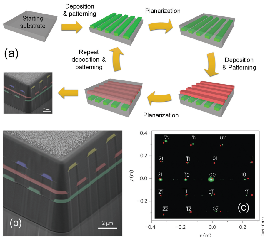
Figure 7. (a) Process flow of multilayer photonic structures in ChG films. (b) Tilted SEM view of a 3-D woodpile photonic crystal showing excellent structural integrity. (c) Diffraction patterns of a collimated 532-nm green laser beam from the photonic crystal. Red dots are diffraction patterns simulated using the Bragg diffraction equation. 11
