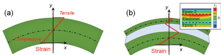
Figure 2. Bending of (a) a simple uniform beam and (b) a sandwiched “Oreo” structure with large elastic mismatch. Strain distributions inside the layers are superimposed on the plots. Inset (b) shows a contour plot of strain distribution inside a trilayer structure computed using the finite-element method.
