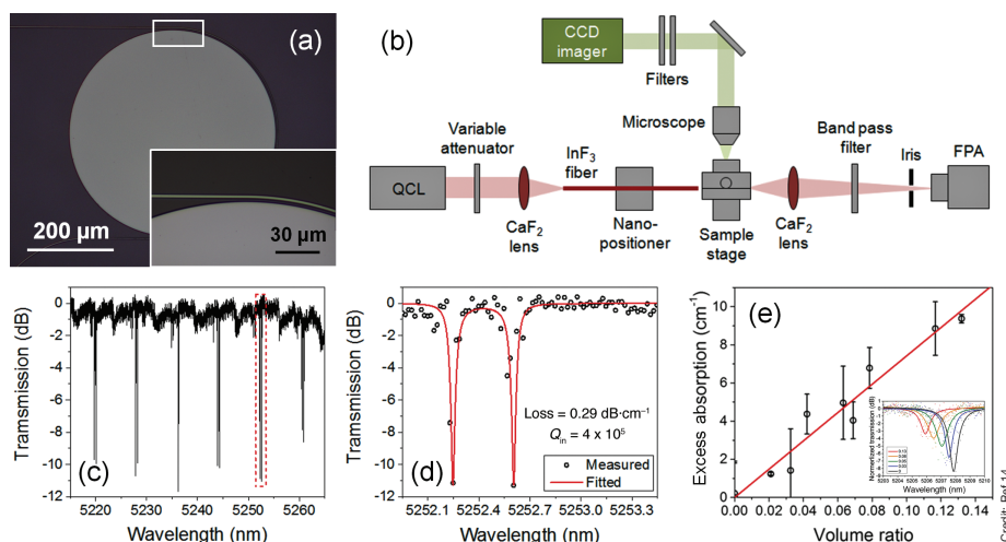
Figure 6. (a) Top-view micrograph of a GSS-on- \text{CaF}_2 microdisk resonator. Inset shows the coupling region between feeding waveguide and microdisk. (b) Experimental setup used to measure mid-IR optical transmission through glass-on- \text{CaF}_2 sensor devices. (c) Mid-IR transmission spectrum of a micro-disk resonator. (d) The same spectrum near an optical resonance at 5252 nm wavelength (red box in (c)). Open circles represent experimental data, whereas the solid line is the doublet-state resonance spectrum fitted by coupled mode theory, which yields an intrinsic Q -factor of 4 \times 10^5 and an equivalent propagation loss of 0.29 \text{ dB}\cdot\text{cm}^{-1} . (e) Optical resonance decreases with increasing ethanol concentration. (images courtesy of Reference 14 authors).
