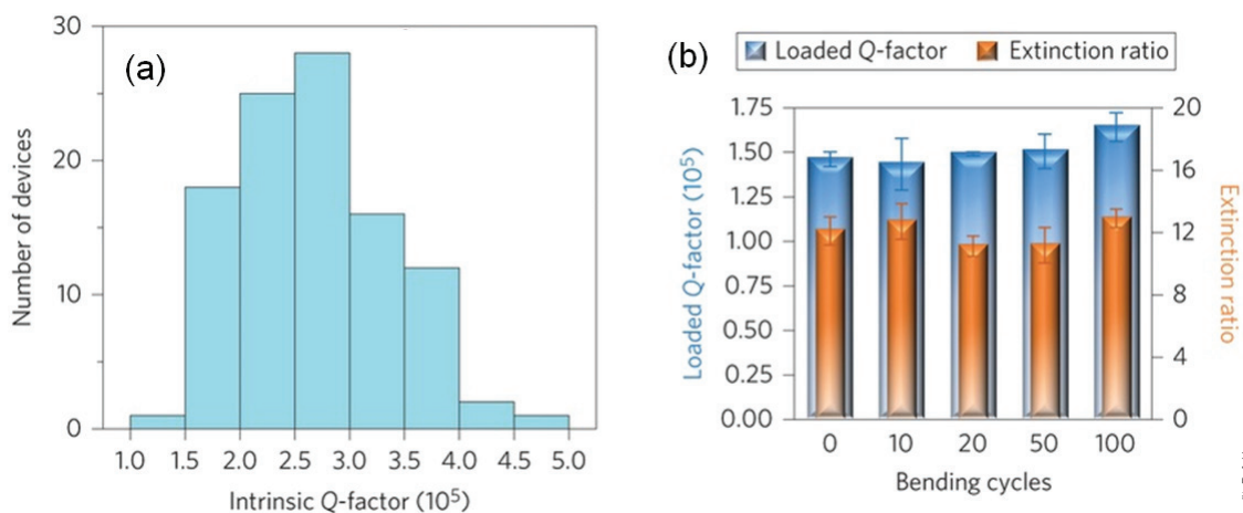
Figure 4. (a) Q-factor distribution measured in flexible microdisk resonators. (b) Q-factors and extinction ratios of the resonator after multiple bending cycles at a bending radius of 0.5 mm. 11
