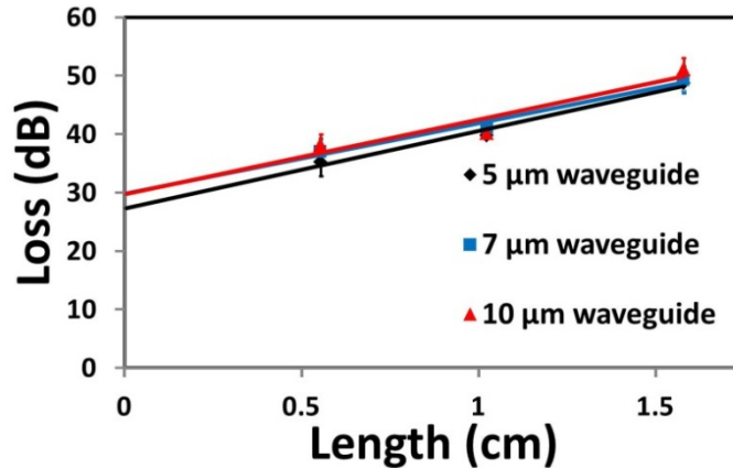
Fig. 8. Total insertion loss of the \text{As}_2\text{Se}_3 waveguides plotted as a function of waveguide lengths. The slopes of the curves yield the propagation loss in the waveguides, while the intercepts with the vertical axis give the coupling loss. The three curves correspond to waveguides of three different widths.
