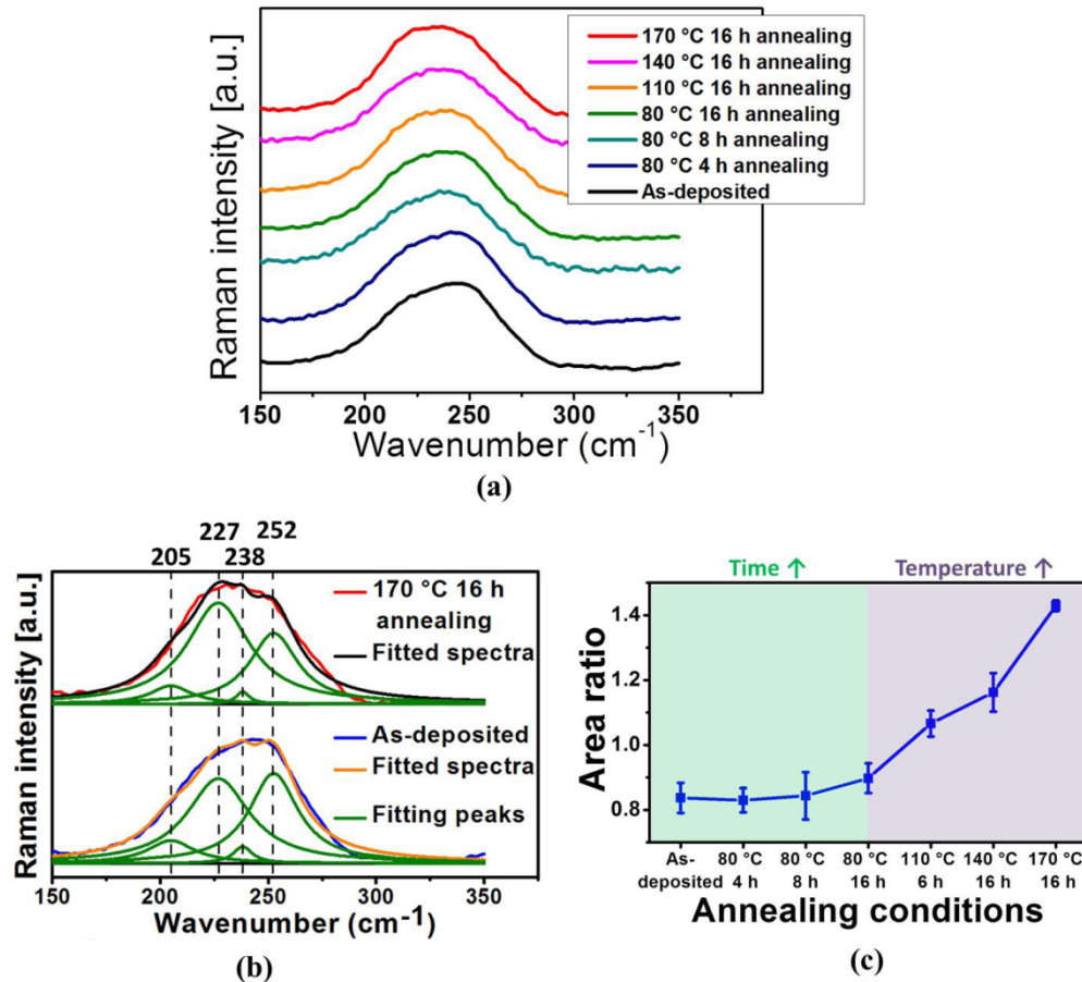
Fig. 4. (a) Raman spectra of spin coated \text{As}_2\text{Se}_3 films under different annealing conditions; the spectra are vertically offset for clarity; (b) Raman spectra from an as-deposited film and a film annealed at 170 °C for 16 hours were fitted by keeping the position of the peaks constant; (c) The peak area ratio, as determined by the area of \text{AsSe}_3 pyramidal unit peaks over the area of peaks corresponding to \text{As}_4\text{Se}_4 unit, Se-Se chain and Se-Se ring, as a function of annealing conditions.
