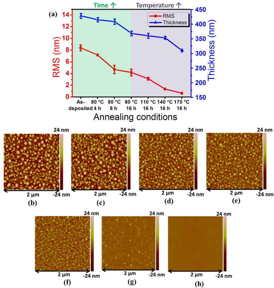
Fig. 2. (a) Thickness and surface roughness of spin coated \text{As}_2\text{Se}_3 glass films annealed at different conditions. (b)-(h) AFM surface profiles ( 2\mu\text{m} \times 2\mu\text{m} ) of glass films annealed at various conditions: (b) as-deposited film; (c) film annealed at 80 °C for 4 hours; (d) film annealed at 80 °C for 8 hours; (e) film annealed at 80 °C for 16 hours; (f) film annealed at 110 °C for 16 hours; (g) film annealed at 140 °C for 16 hours; (h) film annealed at 170 °C for 16 hours.
