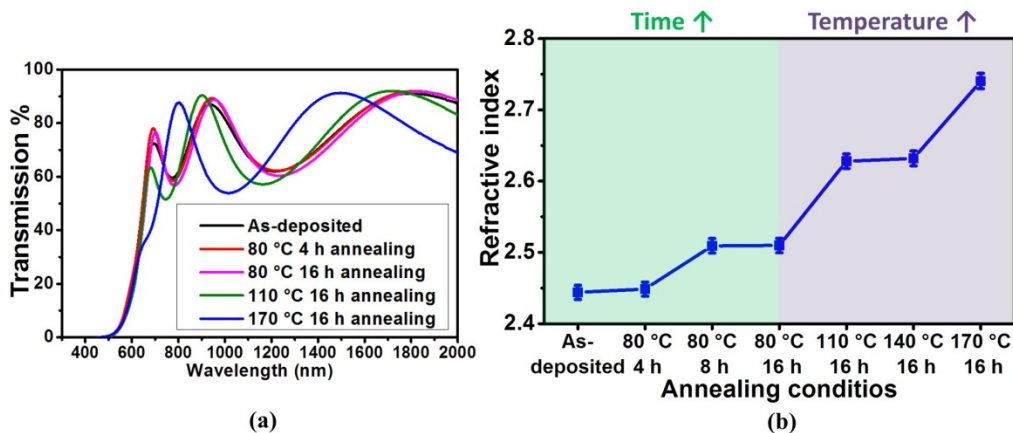
Fig. 6. (a) UV-Vis transmission spectra of spin-coated \text{As}_2\text{Se}_3 films from EDA solution with different annealing conditions. The spectra are not corrected for Fresnel reflection. (b) Effect of annealing on film refractive indices measured at 1500 nm wavelength.
