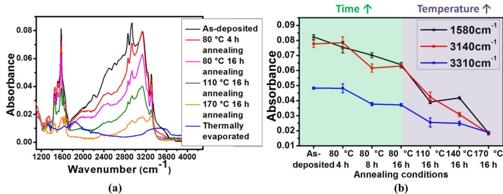
Fig. 5. (a) FTIR absorption spectra of EDA-derived \text{As}_2\text{Se}_3 films vacuum annealed at conditions. (b) Peak absorbance at 1580, 3140 and 3310 \text{cm}^{-1} (due to N-H stretching modes) of EDA-derived \text{As}_2\text{Se}_3 films. The decrease of peak absorbance indicates progressive solvent removal during annealing.
